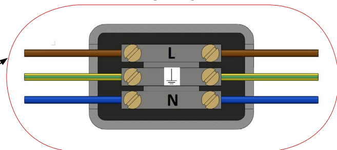
WIRING DIAGRAM
